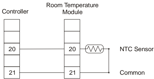
Figure 4: TM-1141-0000 Wiring
