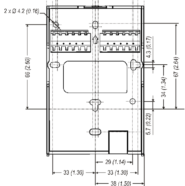
Figure 3: Module Base Dimensions, in. (mm)
