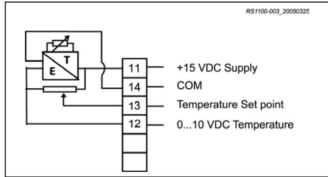
Figure 5: RS-1190-0000 and RS-1190-0005
