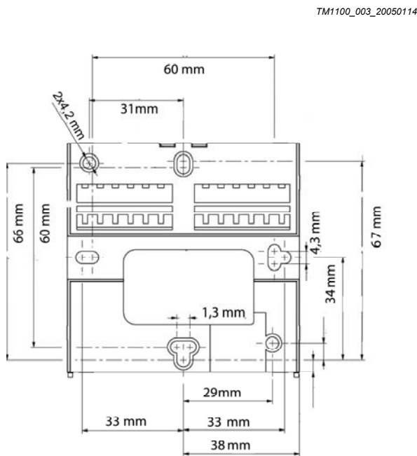
Figure 1: Module Base (Dimensions in mm)
