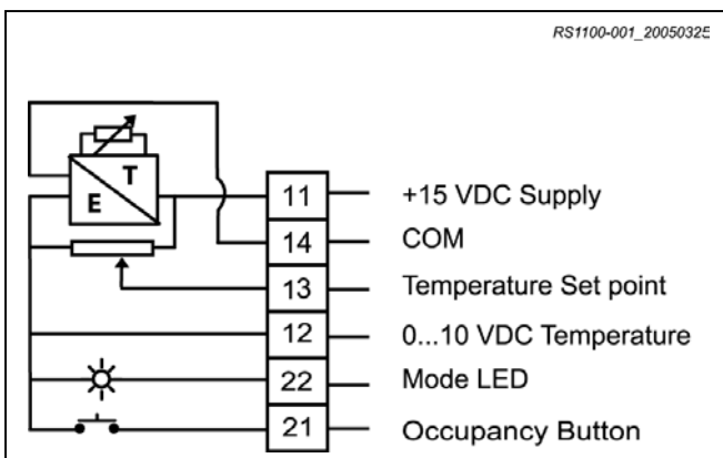
Figure 4: RS-1160-0000 and RS-1160-0005
