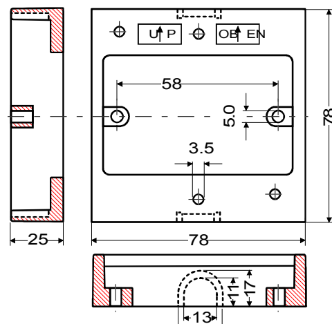
Figure 2: Surface Mounting Base (Dimensions in mm)
